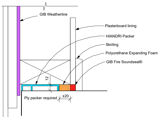
TWO WAY FIRE RATED WALL DETAIL
