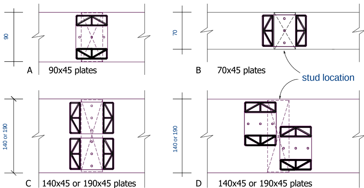
POSITIONING OF HIANDRI PACKERS ON PLATES
